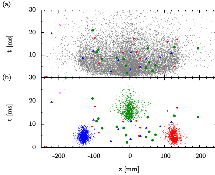
Fig. 5 The two-dimensional time-position ( z, t ) distributions for the escape positions of (a) antihydrogen atoms and (b) mirror-trapped antiprotons after a shutdown of the magnetic trap at t=0 . The dots are the result of numerical simulations of the trajectories of the particles in the magnetic and electric fields of the apparatus. In (b), the green, blue and red distributions correspond to experiments with no applied electric field, an electric field pointing to positive z and an electric field pointing to negative z respectively. The green circles, blue up-pointing triangles and red down-pointing triangles mark the measured times and positions of candidate antihydrogen annihilations in ALPHA for the same electric field configurations. The magenta cross marks the position of the event observed after antihydrogen production using externally-heated positrons.
