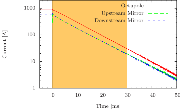
Fig. 2 The measured current flowing in the magnetic minimum trap magnets following a triggered shutdown at t=0 . The dependence is exponential, with time constants 9 ms for the octupole and 8 ms for each of the mirror coils. The orange region shows the 30 ms window over which the search of trapped antihydrogen atoms was conducted.
