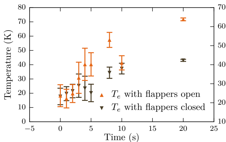
Figure 5.10: Electron temperature measurements made with the flappers open indicated by the orange triangles ( \blacktriangle ) and closed indicated by the brown triangles ( \blacktriangledown ) in February 2017. The error bars show the standard deviation of 8 measurements.
