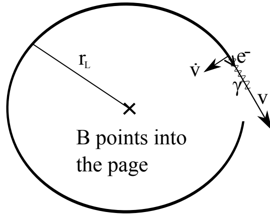
Figure 3.3: Cyclotron motion and radiation of an electron rotating clockwise in a magnetic field pointing into the page.
